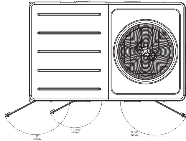
Figure 34. Heat pump - 10 tons standard efficiency - swing diameter for hinged door(s) option
