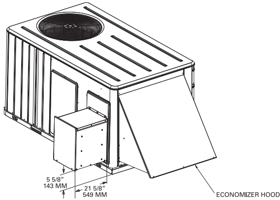
Figure 24. Heat pump - 7½ tons standard efficiency - power exhaust
