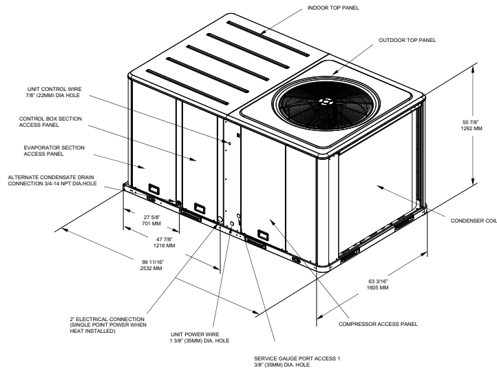
Figure 28. Heat pump - 10 tons standard efficiency - downflow airflow supply/return through the base utilities
