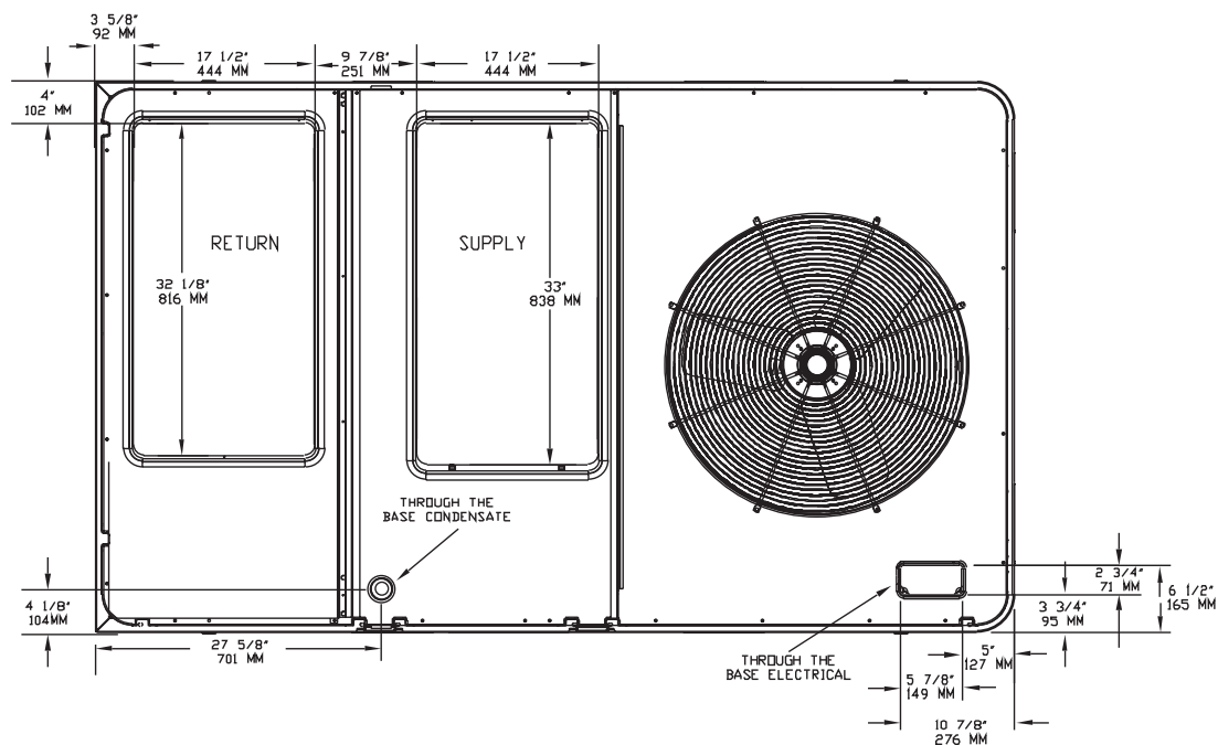
Figure 19. Heat pump - 7½ tons standard efficiency - downflow airflow supply/return through the base utilities
