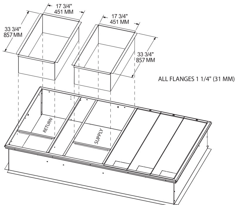
Figure 23. Heat pump - 7½ tons standard efficiency downflow - duct connections field fabricated
