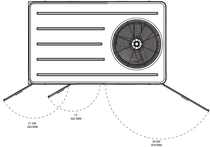
Figure 25. Heat pump - 7½ tons standard efficiency - swing diameter for hinged door(s) option
