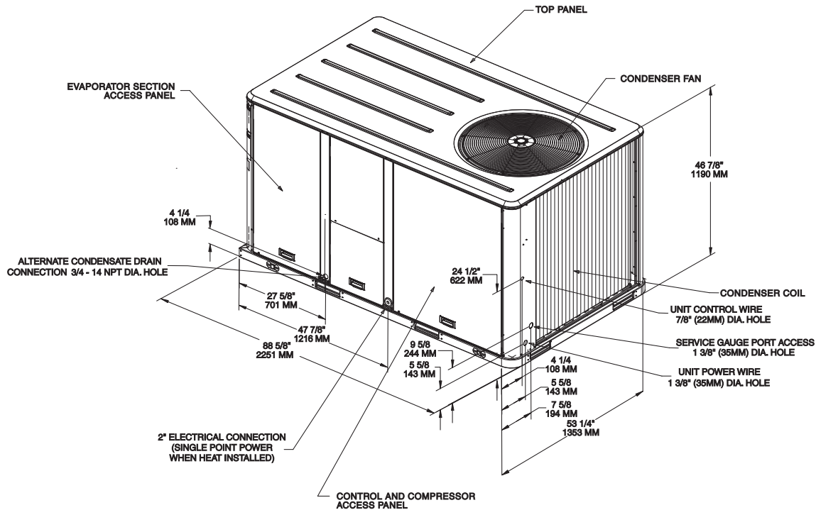
Figure 19. Heat pump - 7½ tons standard efficiency - downflow airflow supply/return through the base utilities
