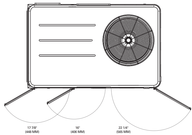
Figure 8. Heat pump - 3-4 tons standard efficiency - swing diameter for hinged door(s) option
