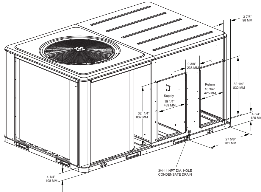
Figure 30. Heat pump - 10 tons standard efficiency - unit clearance and roof opening
