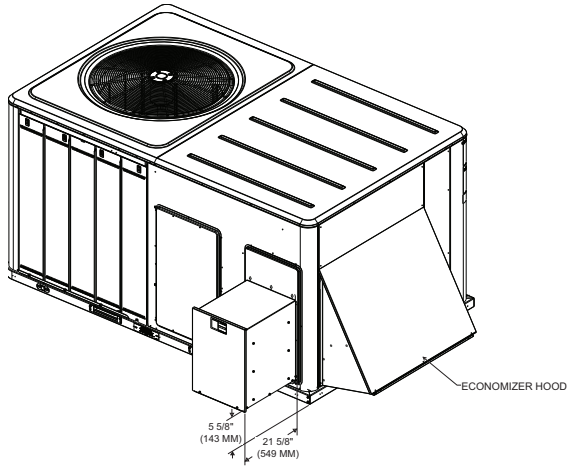
Figure 33. Heat pump - 10 tons standard efficiency power exhaust
