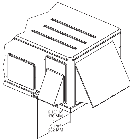
Figure 9. Heat pump 3-4 tons standard efficiency - economizer & barometric relief damper hood
