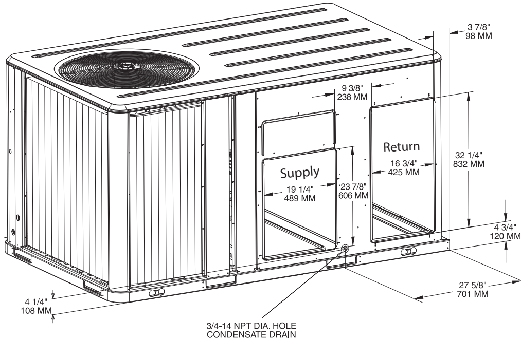
Figure 21. Heat pump - 7½ tons standard efficiency - unit clearance and roof opening
