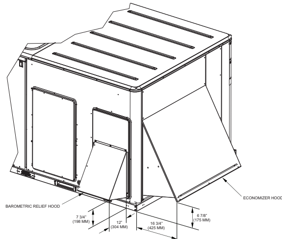
Figure 35. Heat pump - 10 tons standard efficiency economizer, manual or motorized fresh air damper
