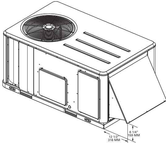
Figure 7. Heat pump - 3-4 tons standard efficiency - economizer, manual or motorized fresh air damper
