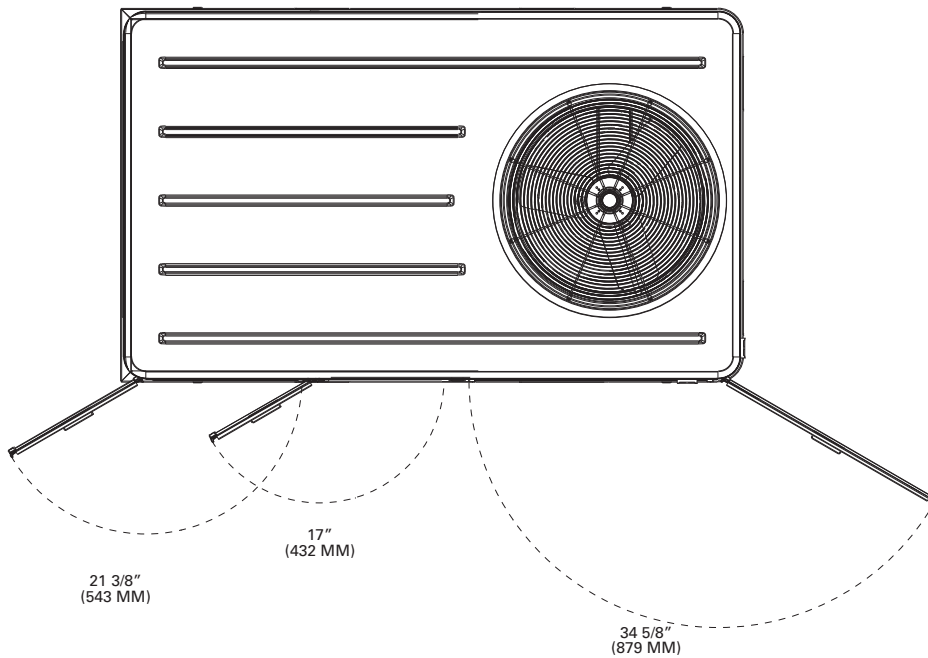
Figure 17. Heat pumps - 5-6 tons - swing diameter for hinged door(s) option
