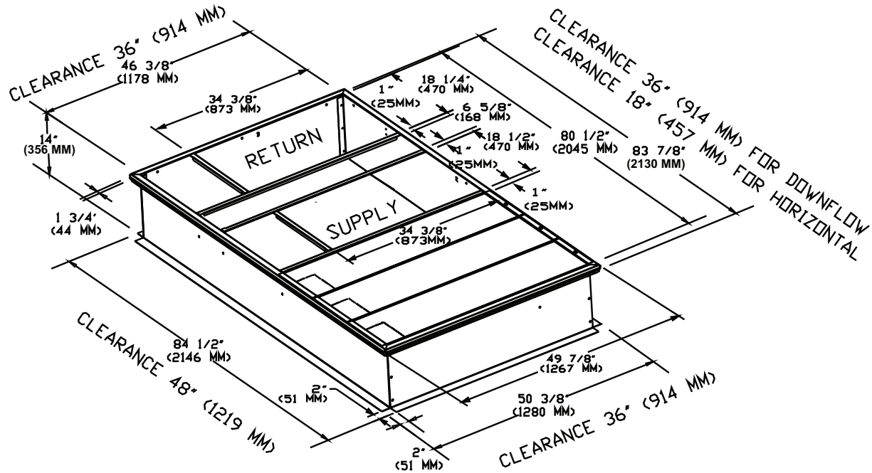
Figure 23. Heat pump - 7½ tons standard efficiency downflow - duct connections field fabricated
